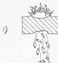
FIGURE 41. Scabbing effect. 1) Plastic explosive placed directly against target. 2) Scabbing effect during detonation.
