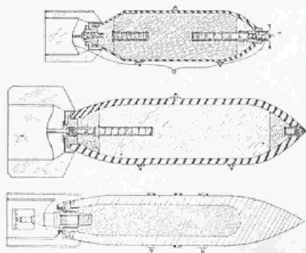
FIGURE 128. Dropped munitions (bombs for aircraft).
