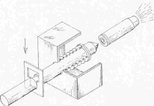
FIGURE 57. Silhouette cocked striker release device.
