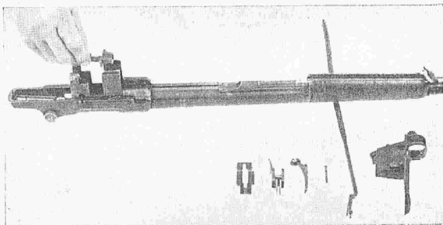
PLATE 9. LIFTING OUT FOLLOWER
