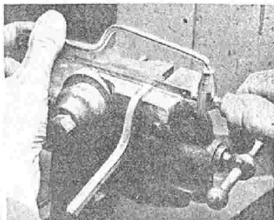
Now start to form the teeth by making a row of shallow saw slots, about \frac{1}{8} in. apart, on the surface of the short leg of the tool
