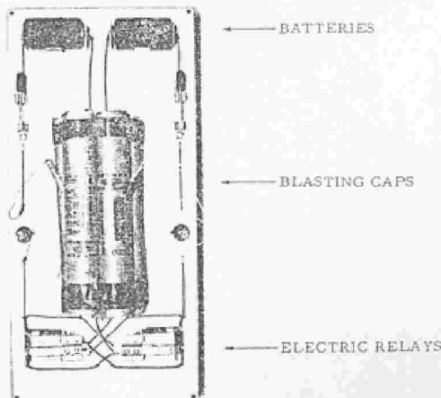
FIGURE 104. Long delay, collapsing, and booby trapped bomb.
