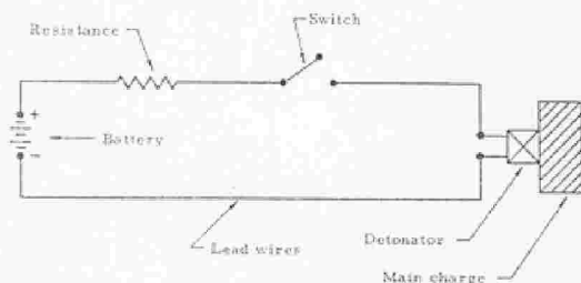
FIGURE 53. Basic electric circuit.
