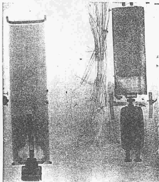
FIGURE 182. X-ray photo of suspected package. Note blasting caps in center and upper right of picture.
