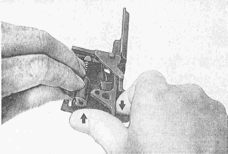
PLATE 20. REPLACEMENT OF THE TRIGGER ASSEMBLY, HAMMER SPRING HOUSING, HAMMER SPRING, AND HAMMER SPRING PLUNGER
