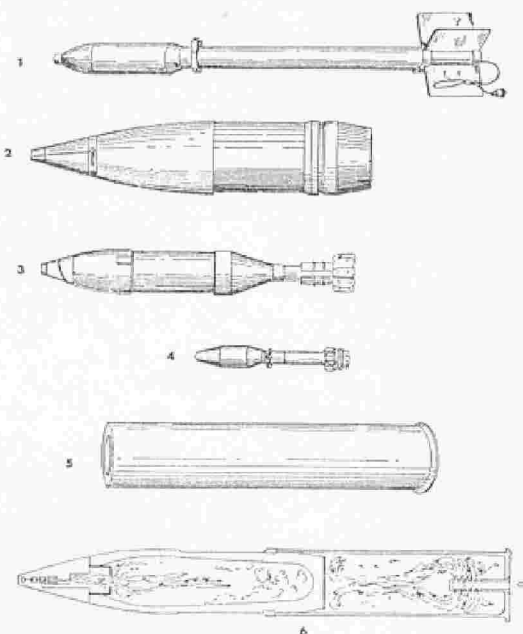
FIGURE 126. Projected munitions, military projectiles, etc.
