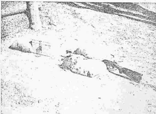
FIGURE 149. Shotgun de-armor in position for attack on suspected package. Stand-off distance, approximately twelve inches.
