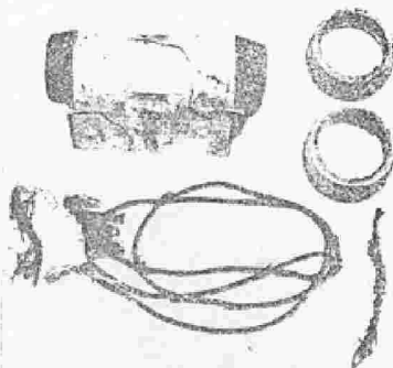
FIGURE 164. Evidence gathered at the scene of pipe bombing. (Courtesy Federal Bureau of Investigation)
