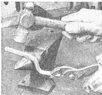
In making the bottoming tool—used to smooth the bottom of the gouged-out slot in a rifle stock—first heat the longer leg and bend it
