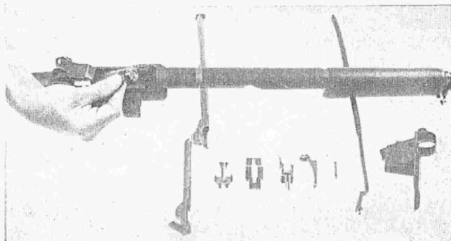
Figure 1. Removing Bolt PLATE II. DISASSEMBLY OF BOLT
