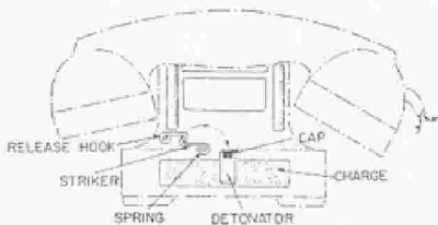
FIGURE 87. Telephone booby trap.
