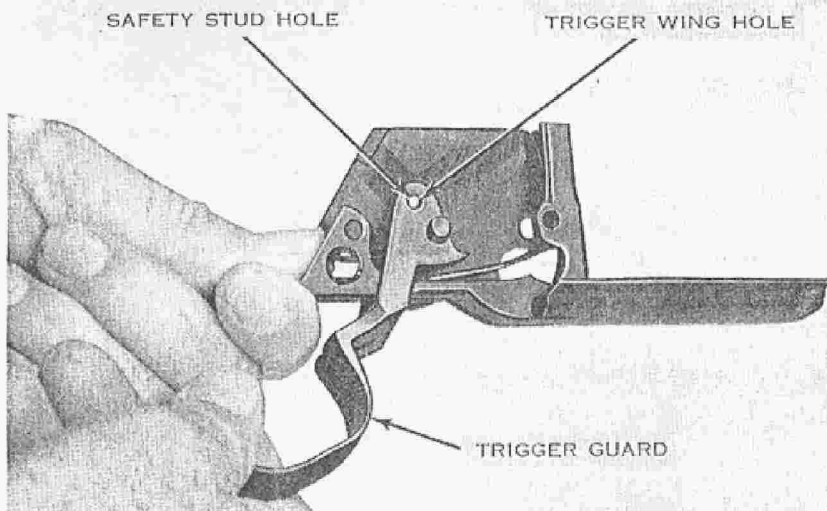
PLATE 17. REMOVING THE TRIGGER GUARD
