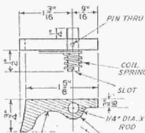
FIG. 4 HAMMER (1/4" STOCK)
