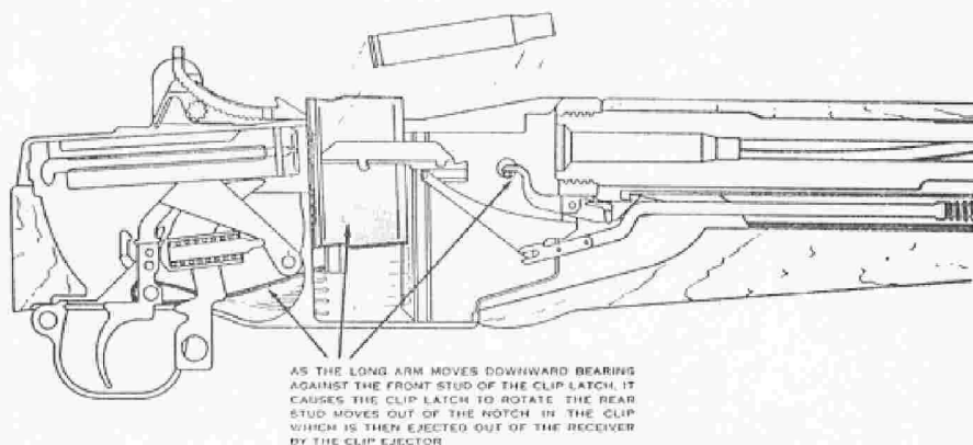
PLATE 24. ACTION FOLLOWING THE FIRING OF THE LAST ROUND
