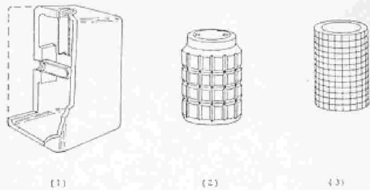
FIGURE 32. Fragmentation effect, internal charges. 1) Solid case, 2) Pressurized, 3) Wire wrapped.
