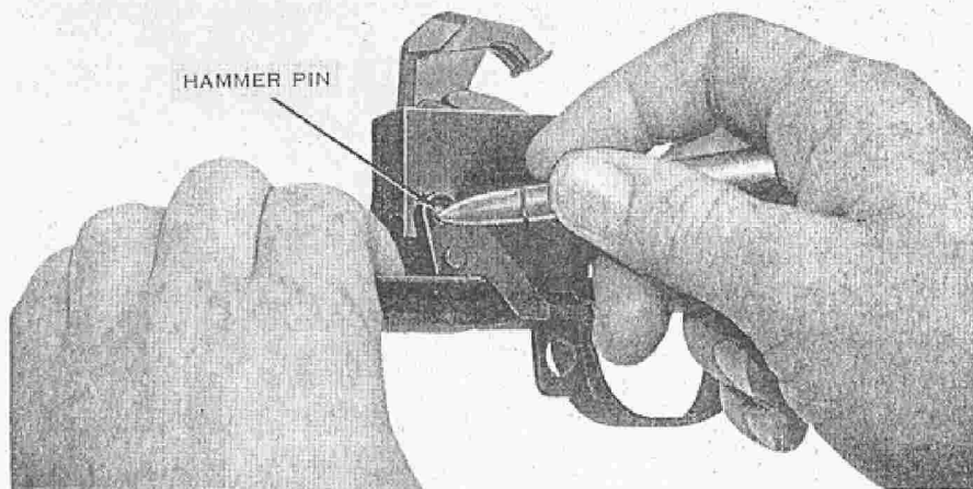
PLATE 15. REMOVING THE HAMMER PIN AND HAMMER
