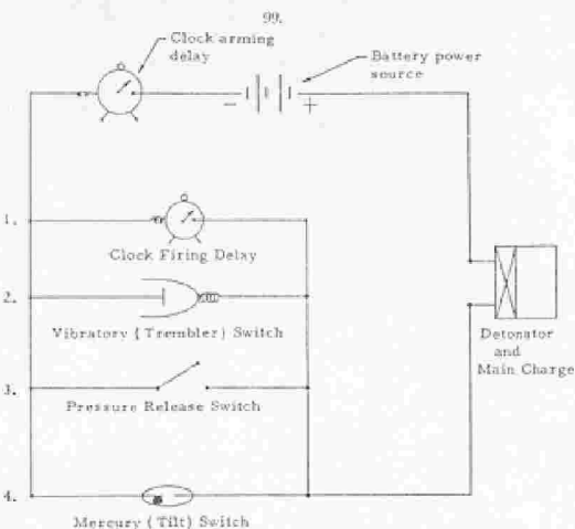
FIGURE 55. Long delay, anti-disturbance, booby trapped circuit.
