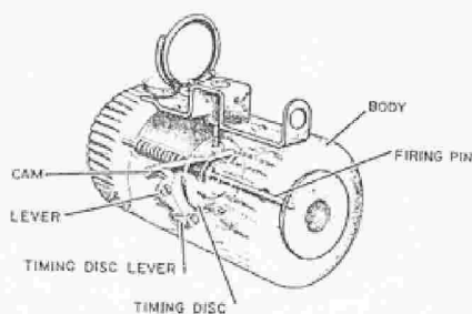
FIGURE 58. Clockwork timing disc.
