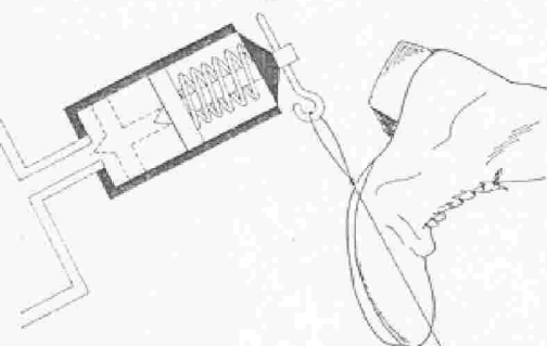
FIGURE 56. Cocked firing pin (pull initiated) device.
