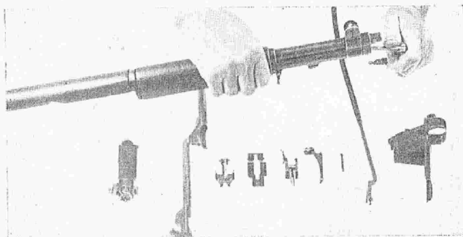
PLATE 12. REMOVING GAS CYLINDER LOCK SCREW
