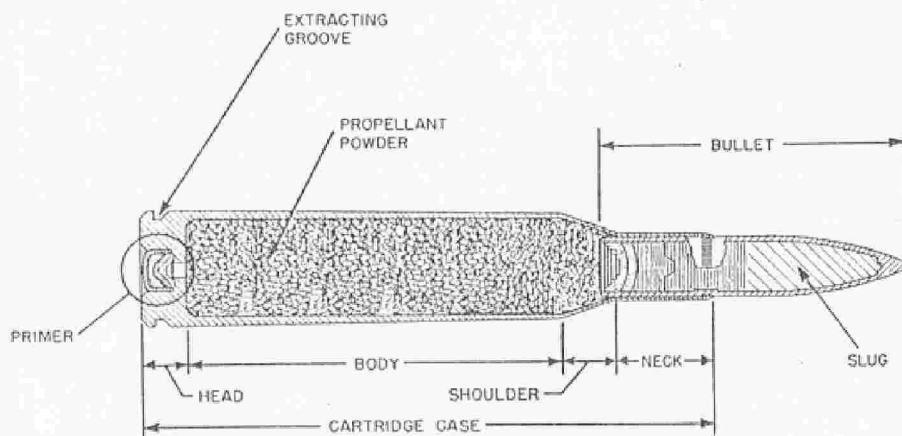
PLATE 31. PARTS OF THE CALIBER .30 ROUND
