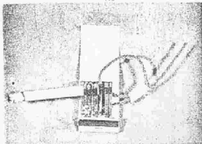
FIGURE 67. Cigarette and matchbook delay device.
