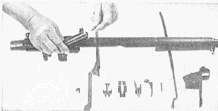
Figure 5. Removing Ejector and Ejector Spring PLATE 11. DISASSEMBLY OF BOLT (Continued)
