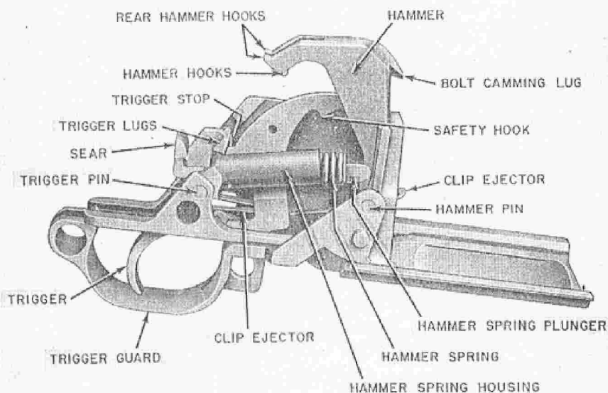
PLATE 25. TRIGGER HOUSING GROUP
