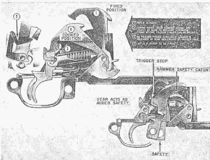
PLATE 26. FUNCTIONING OF THE TRIGGER HOUSING GROUP
