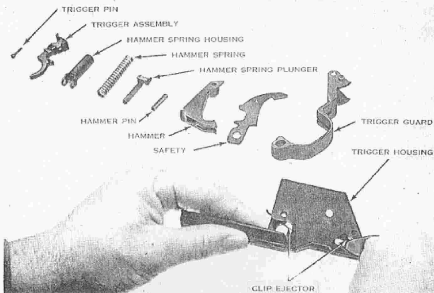
PLATE 18. REMOVING THE CLIP EJECTOR
