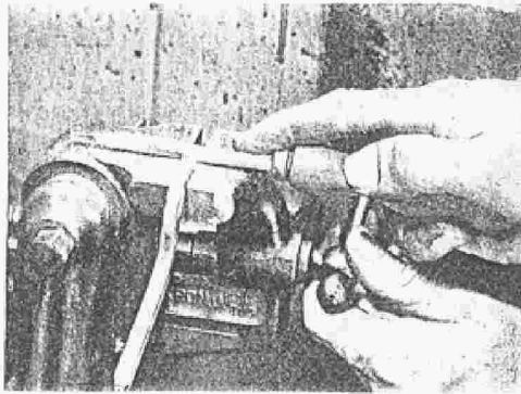
Shape the teeth with a triangular file, giving the front surface of each tooth a backward rake. [See sketch 5-B, on next page.]
