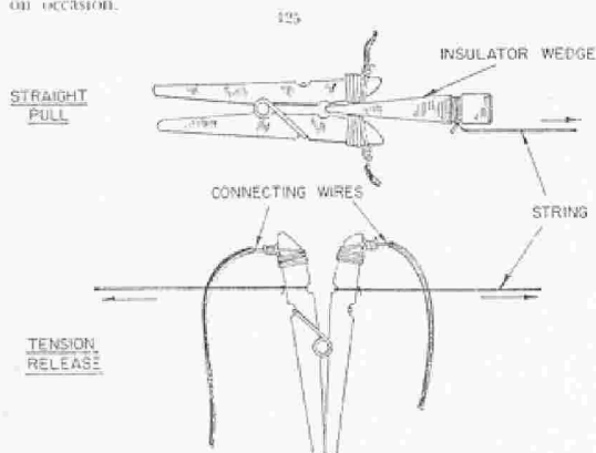
FIGURE 75. Clothes pin electric switching devices.
