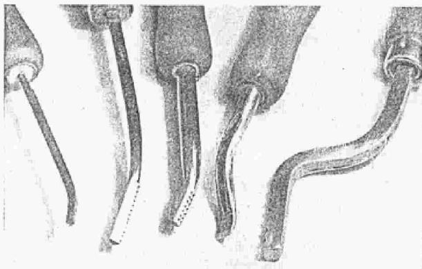
Business ends of homemade gun tools. Left to right: bent-file smoothing tool for checkering, checkering layout tool, two-row checkering tool, carving gouge, and bolt-taming tool
