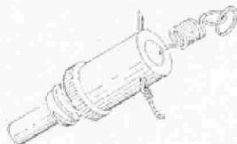
FIGURE 74. M-2 pull friction device.
