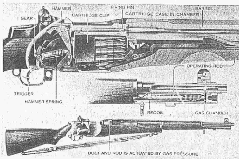
Basic Functioning of the Garand
