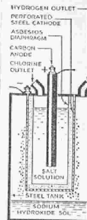
Experimental set-up for extracting chlorine, hydrogen, and sodium hydroxide (lye) from brine. Drawing shows the Nelson cell used commercially
