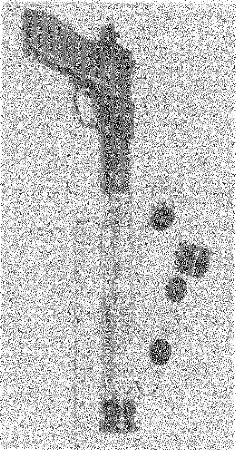
Here is a stripped silencer from a kit designed in the 1980s by RFP, Inc. Mounted on an S&W 39, this silencer is a wiper design using baffles, chambers, and an unusual ported swirl section. (Photo courtesy of J. David Tribby, Silencers in the 1980s )
