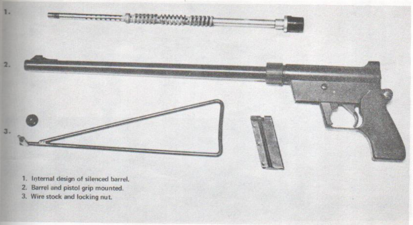
A product literature photo showing parts for the R. P. B. suppressed AR7 survival rifle.
