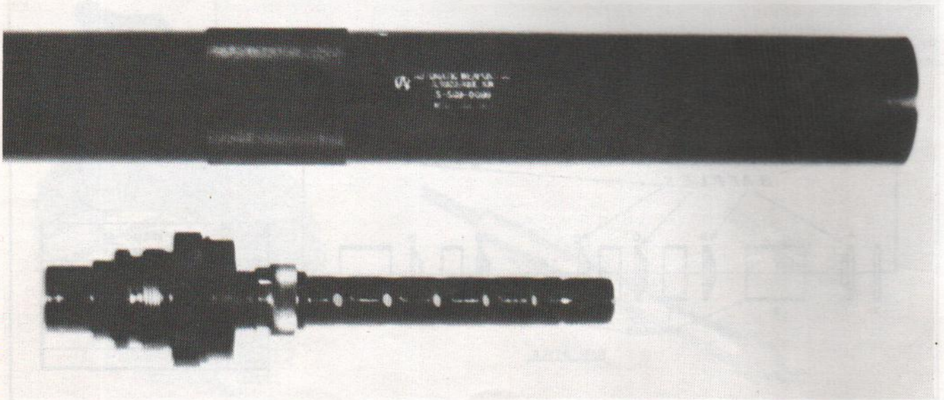
Phil Dater's SG9 suppressor with adapter for the Sten. This same basic suppressor may be used with a variety of 9mm weapons.
