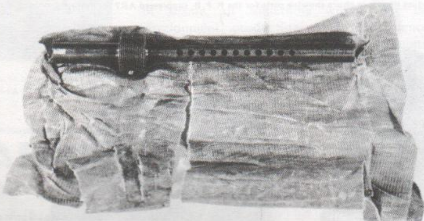
An original CIA SMG barrel, ported for suppressor use—possibly for a S & W M76 or an M3A1. The waterproofed wrapping is shown too.
