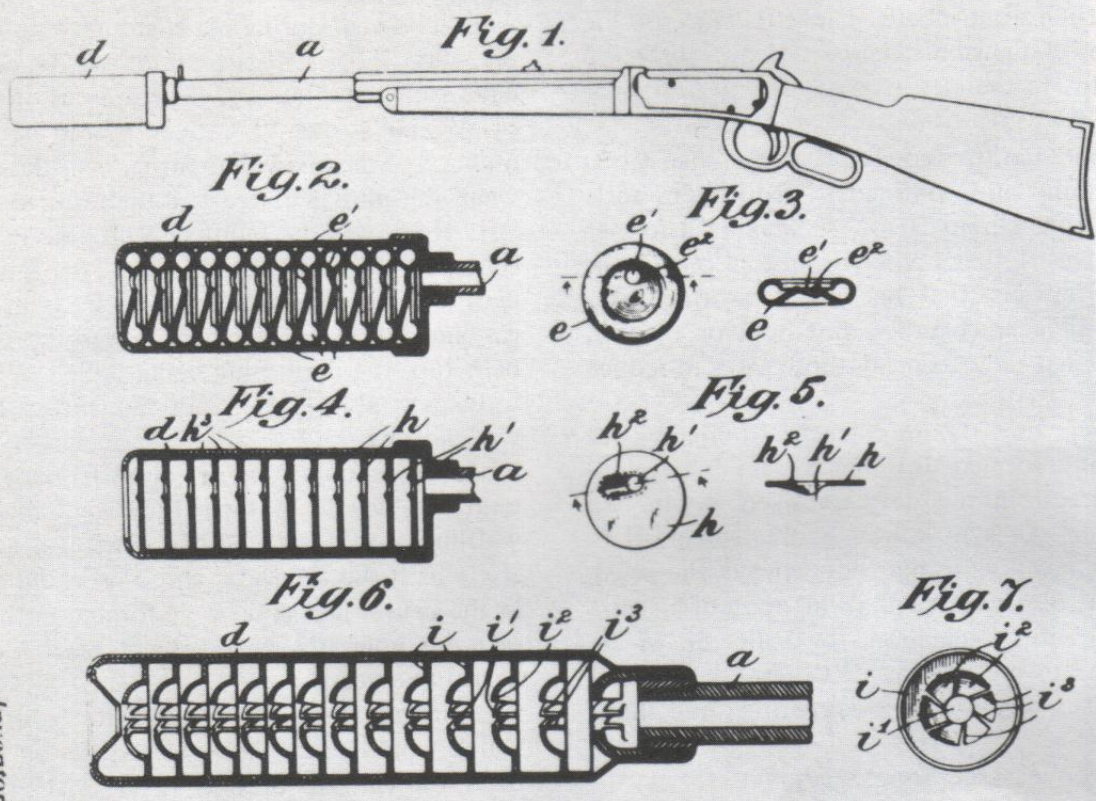
The patent illustration for H. P. Maxim's first truly successful silencer.
