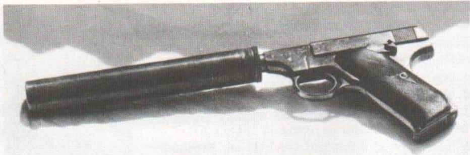
The .22 caliber sealed suppressor on a Colt Woodsman.
