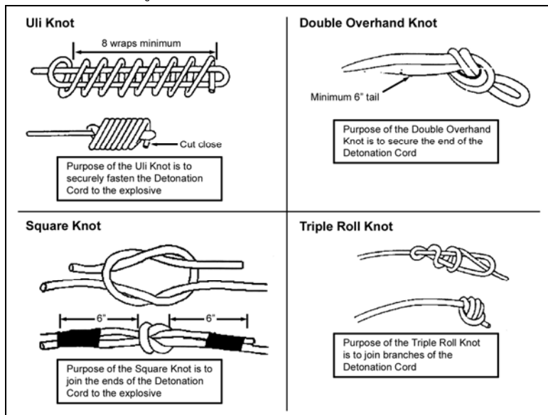
Figure 13-5. VARIOUS JOINING KNOTS USED IN DEMOLITIONS
