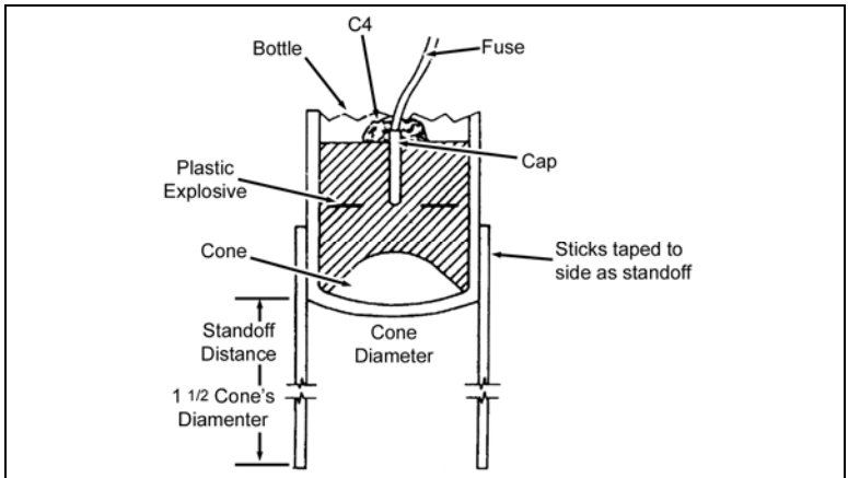
Figure 13-2. IMPROVISED SHAPED CHARGE
