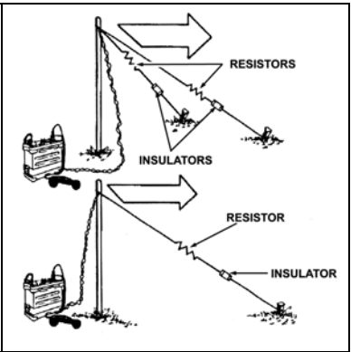
Figure 7-13. SLOPING VEE ANTENNA
