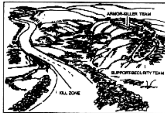
Figure 5-7. Antiarmor ambush.
