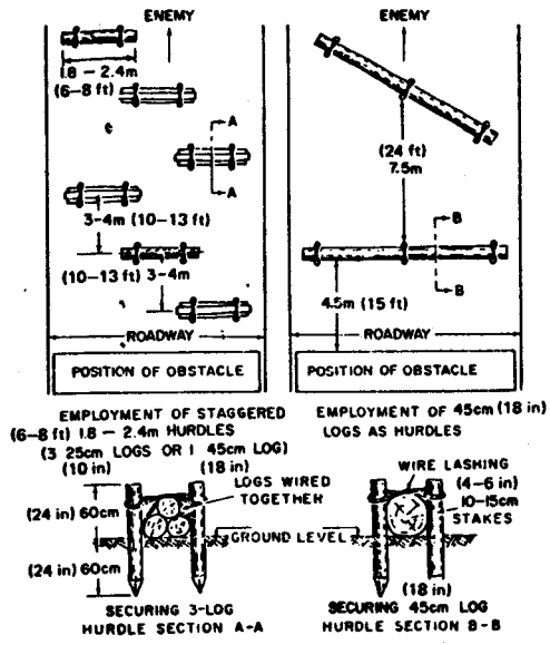
Figure 8 Type Log Hurdles
