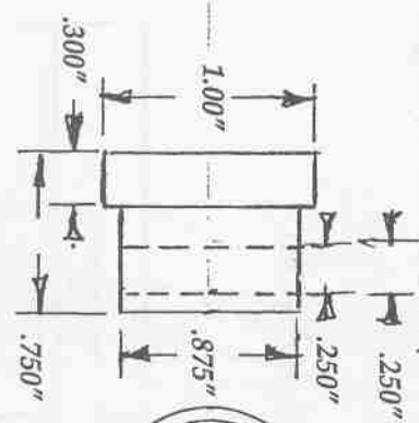
BRECH PLUG
