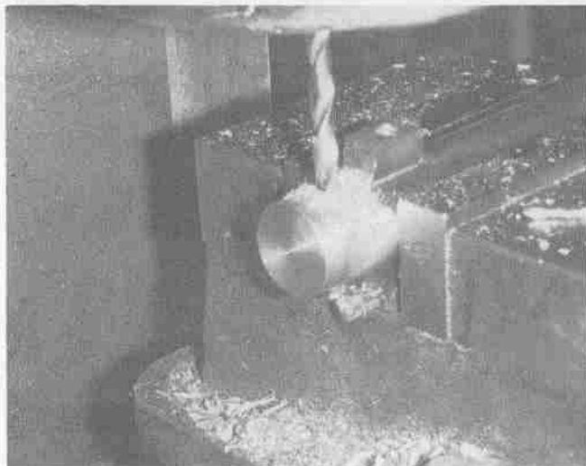
The hole for the breech plug retaining pin is drilled through both receiver and plug simultaneously.
