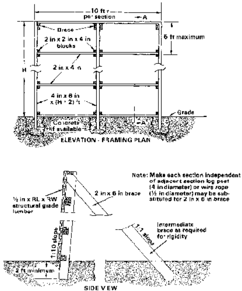
Typical standoff framing with dimensioned wood triggering screen
