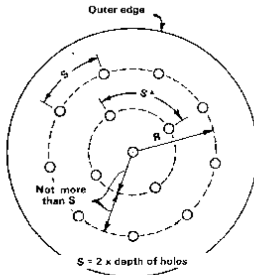
Boreholes for circular positions
