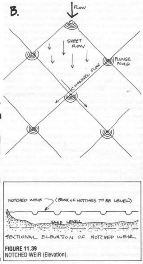
FIGURE 11.38. A BRAIDED STREAM. A natural braid occurs in sand beds at the centre of flood plains. B NOTCHED WEIRS can spread flood braiding across a full flood plain; hatched areas show absorption areas where trees and shrubs will grow (see detail). C. Details of braid patterns in sand, notched weir to initiate braiding in sandy rivers.
