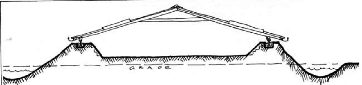
FIGURE 9.19 EARTH-COMPACTED WALL CONSTRUCTION Using modern earthmoving equipment, a house or barn of this type can be completed in about three days.
