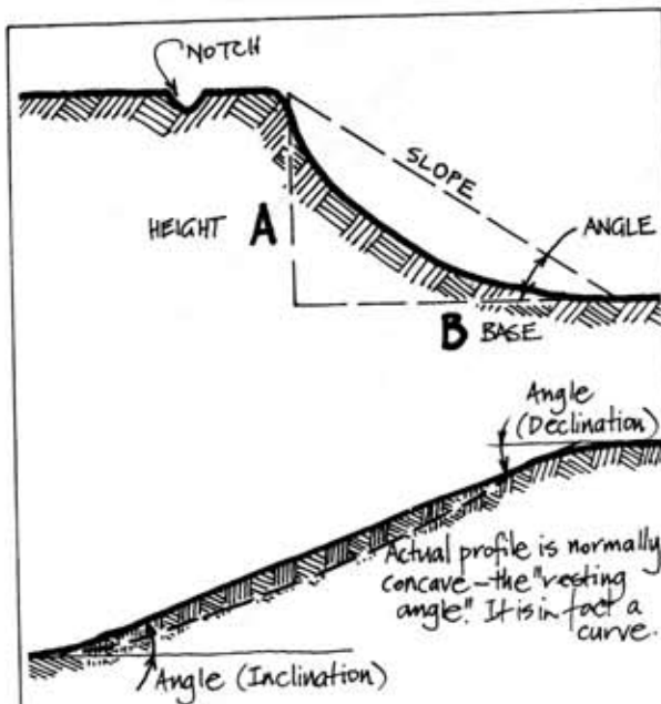
FIGURE 9.4 CONCAVE SLOPES
