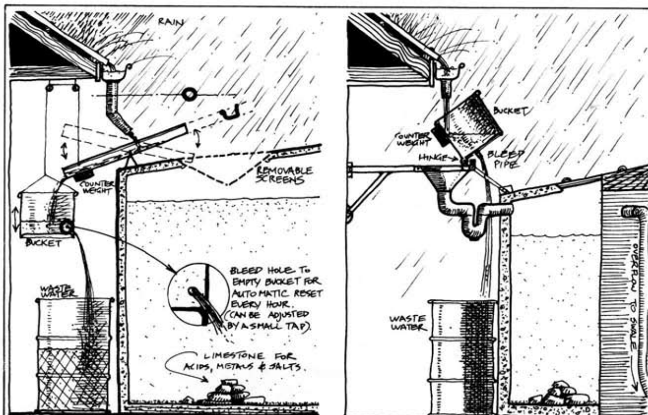
FIGURE 7.21 METHODS OF REJECTION OF FIRST WATER FLOW OFF A ROOF. The first rains wash the roof, and are rejected; these systems automatically reset when empty.
