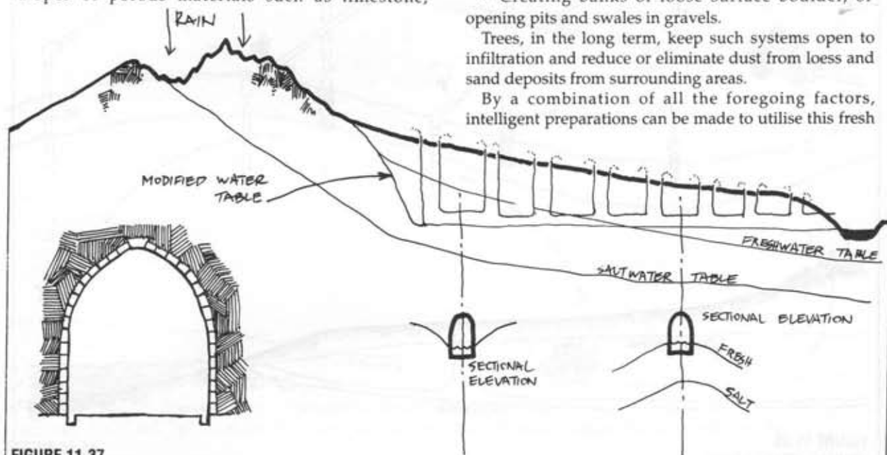
FIGURE 11.37 QUANATS.
