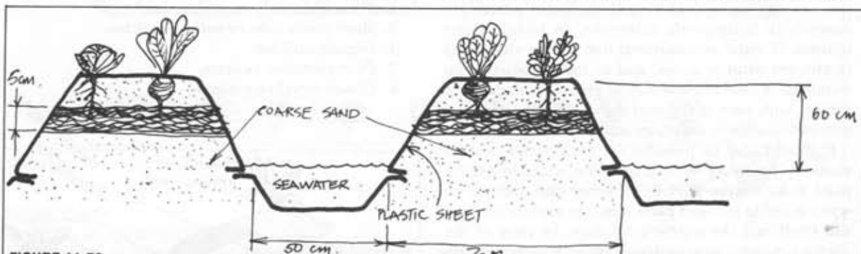
FIGURE 11.72 SEA OR BRACKISH WATER FOR GARDEN IRRIGATION. Extremely salty water or seawater will evaporate under plastic to root-water plants via sand, peat layer. Warranted only in extreme
