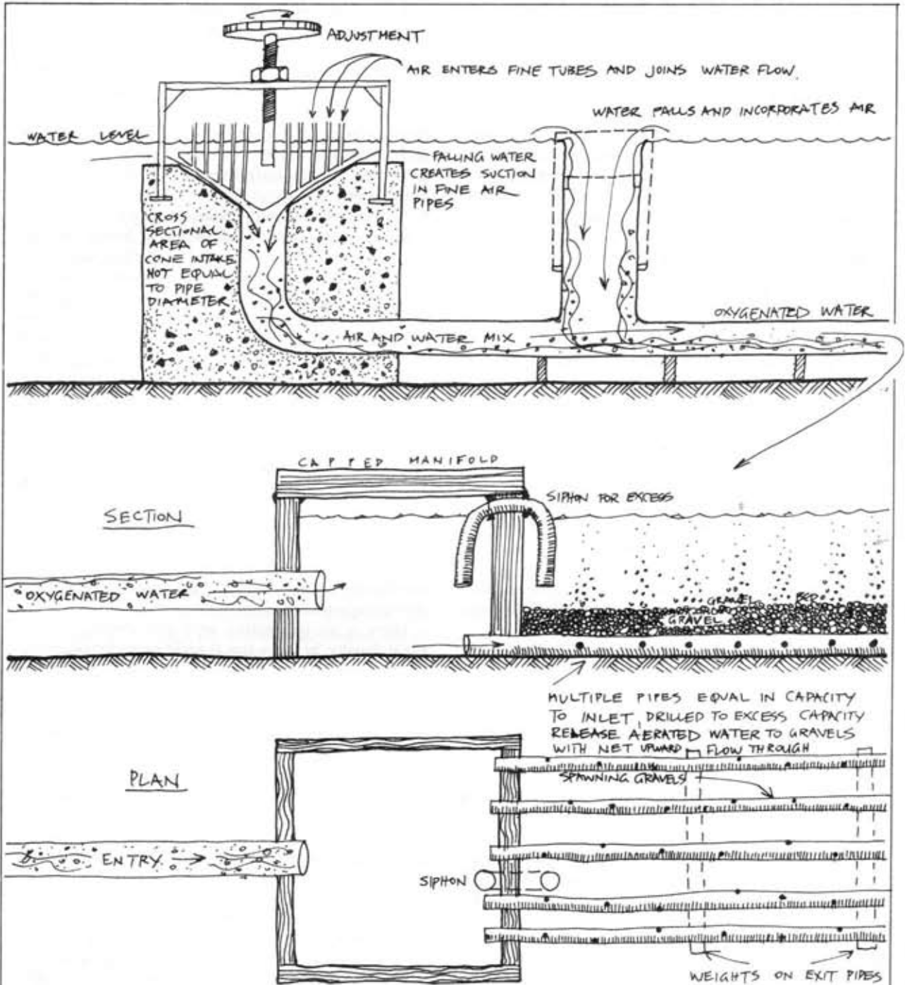
FIGURE 13.7 CONE AERATOR
