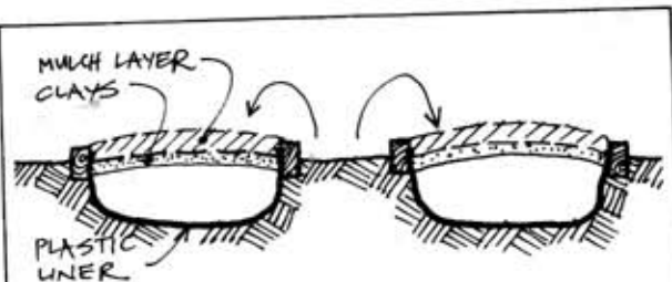
FIGURE 8.7 LAYING PLASTIC IN DEEP SANDS
