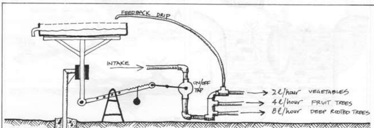
FIGURE 11.73 AUTOMATIC IRRIGATION (my schematic). Pan evaporation is here used to switch on a manifold of trickle irrigation lines; feedback and rainfall is accounted for; a set period of irrigation resets the system.
