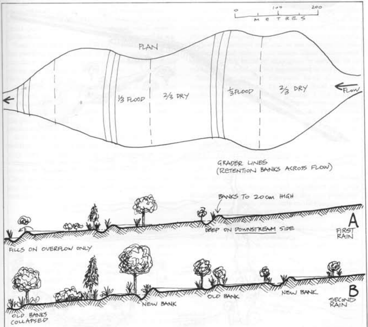
FIGURE 11.20 REVEGETATION OF SCALDS.
