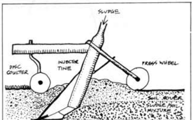
FIGURE 12.16 SLURRY INJECTION IN GRASSLANDS.
