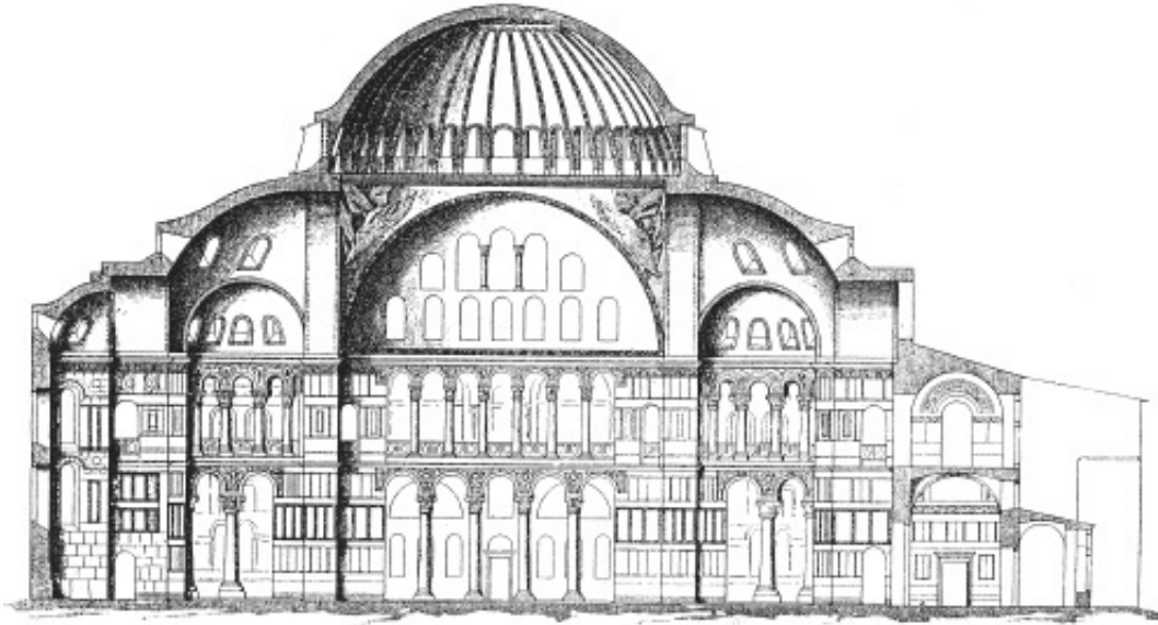
St. Sophia in cross-section
