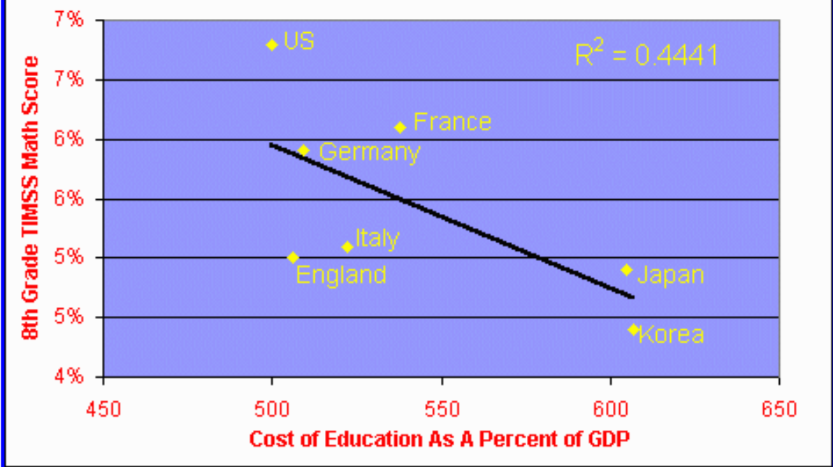
TIMSS Scores Increase 40 Points For Each 1% of GDP Decrease in Education Spending
