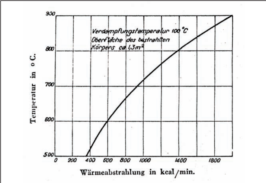
Document 47: Diagram of radiation from the walls of a muffle onto a body in a crematorium oven as a function of temperature. From: Schlöpfer 1938, p. 153.
