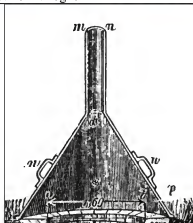
Illustration 12.10: Funnel and "chimney" of the Feist oven.
