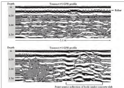
Illustration 8.47: “Ground-penetrating radar reflection profiles of garage floor with Transect 1 showing the rebar embedded in the concrete slab and no indications of a buried body, while Transect 2 shows the point source reflection of the buried body directly under the area where the floor had been repaired.
